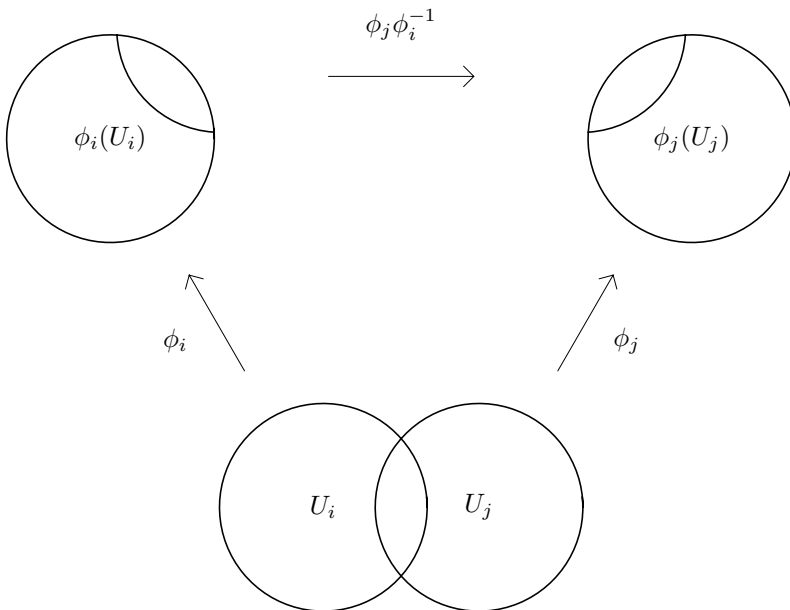
Figure 8.3.1. A coordinate change
